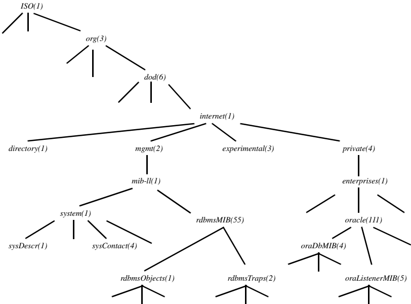
Figure 1-2 The MIB Hierarchy
