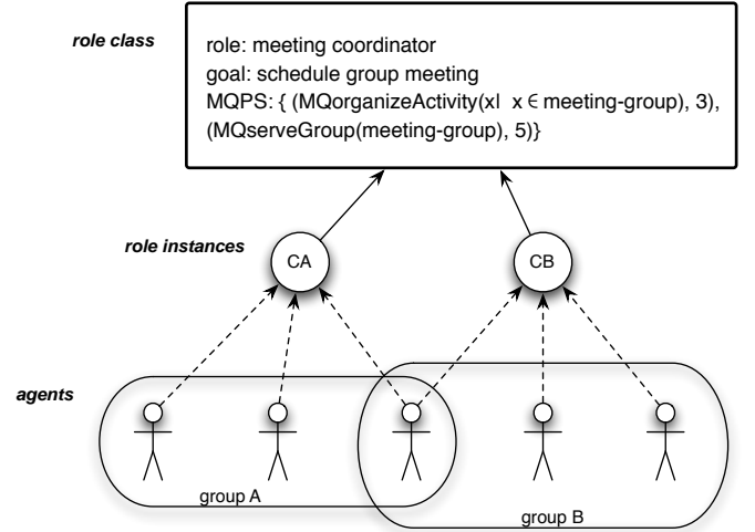
Fig. 5. Meeting coordinator role example
