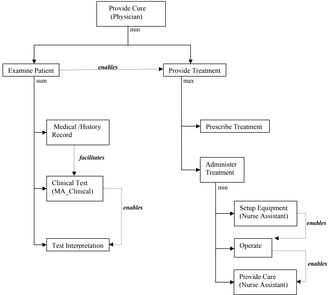
Fig. 6. Plan tree for goal Provide Cure in RTÆMS representation
