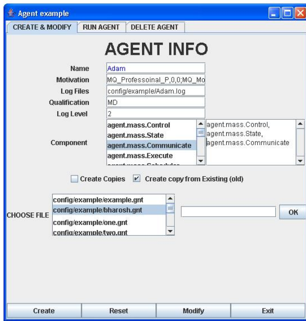
Fig. 8. Automatic agent generation interface
