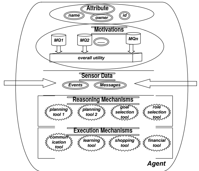
Fig. 7. An general agent architecture
