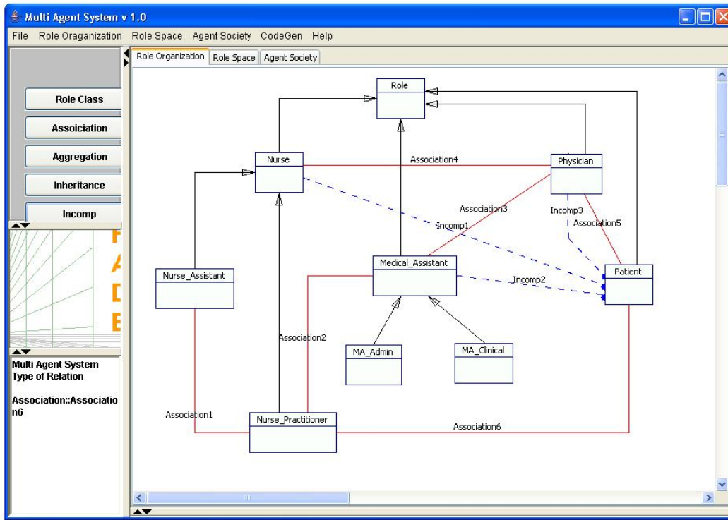
Fig. 9. RADE interface for creating roles
