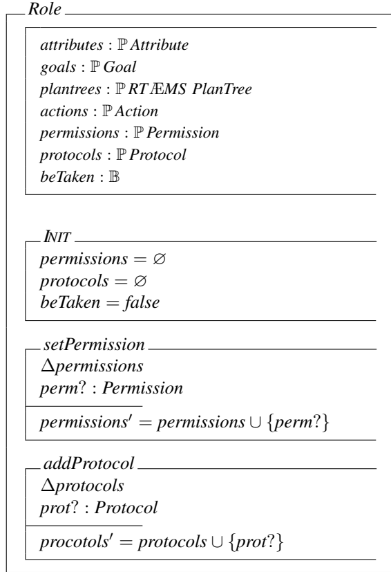
Fig. 4. Definition of role
