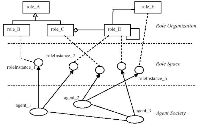
Fig. 1. A generic model of role-based open multi-agent systems (adapted from [30])
