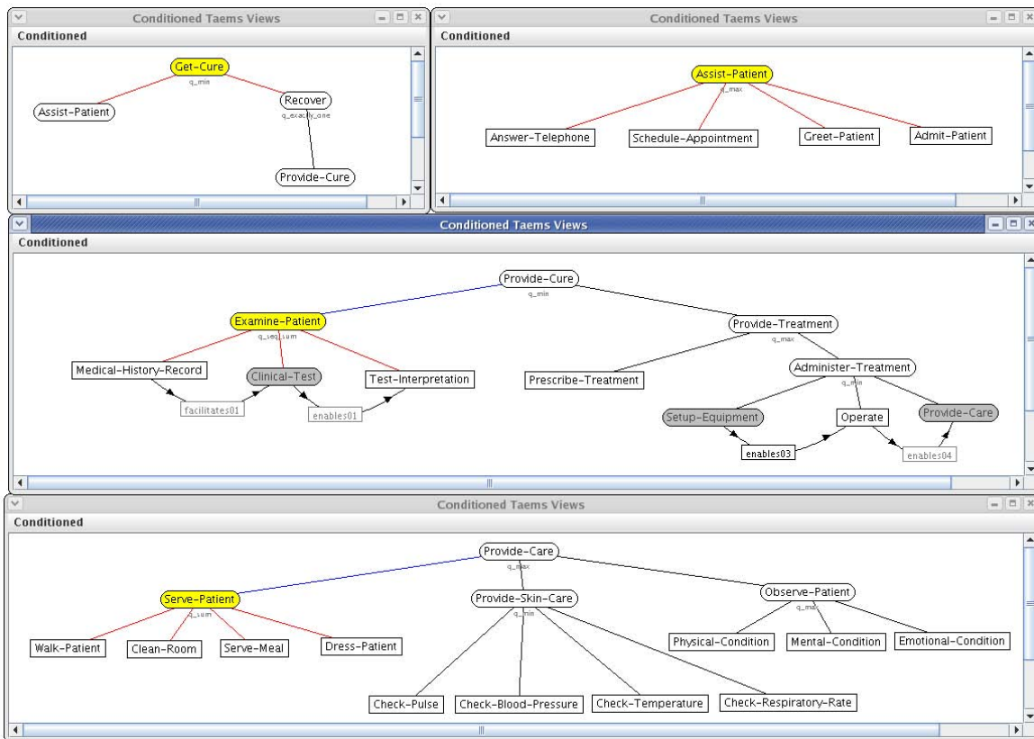
Fig. 10. Plan tree definitions for multiple goals
