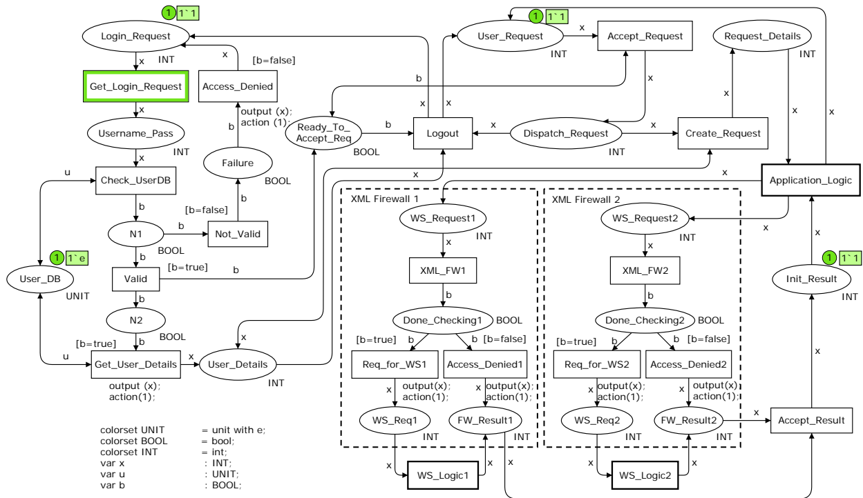
Figure 3 CPN model of an application that invokes two web services
